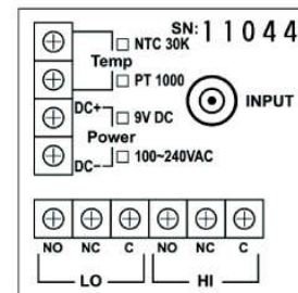
Rear Panel Connection
